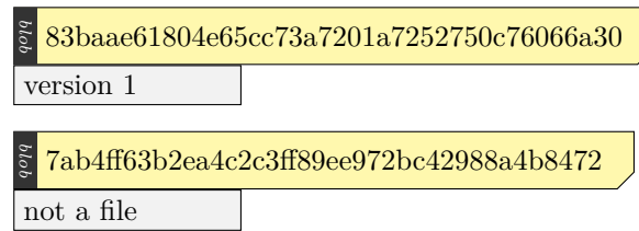
Figure 2.2: Two Git blobs
