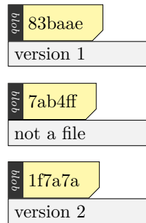
Figure 2.3: Three Git blobs
